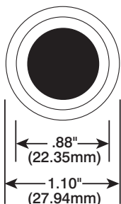
ROUND HOLE
