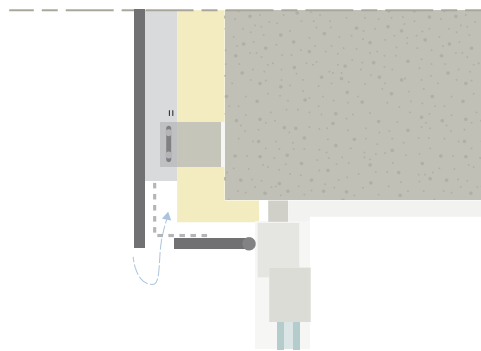
Figure 15: Window Sill
